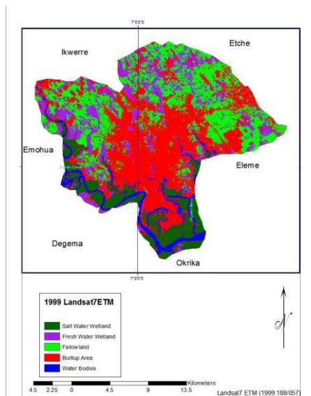
Figure 5: 1999 Landsat 7 ETM
