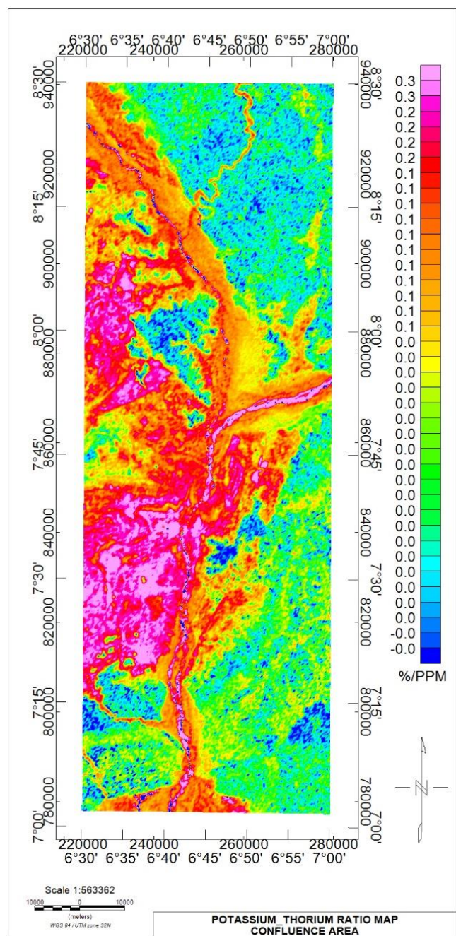
Figure 7: Potassium-Thorium Ratio map
