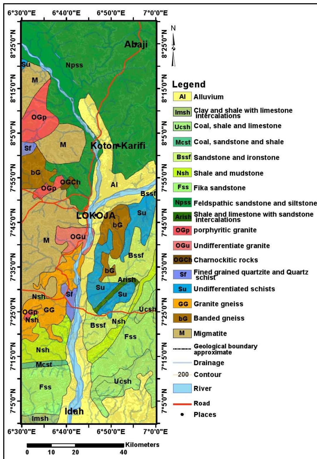
Figure 2: Geological map of Study Area (adapted from NGSA, 2009)
