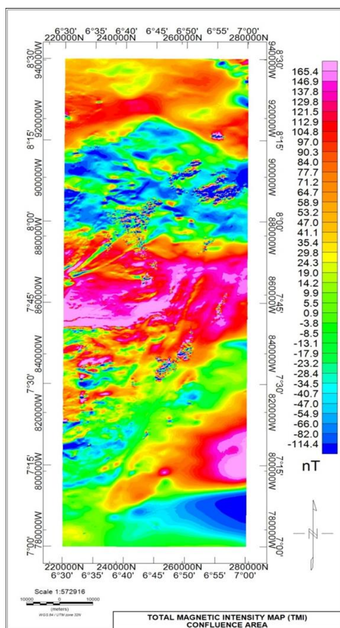
Figure 3: Total magnetic Intensity Map
