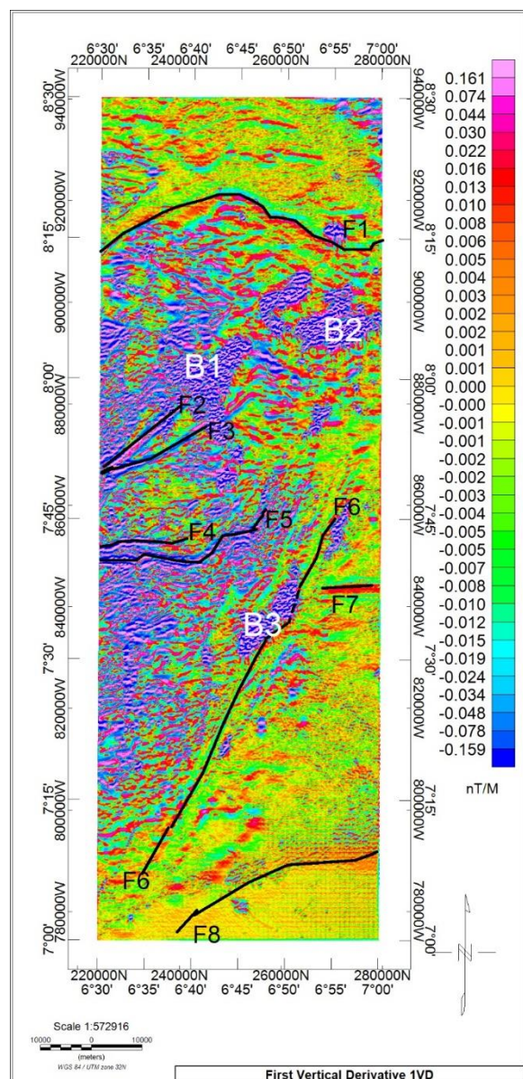
Figure 5: First Vertical Derivative Map (1VD)
