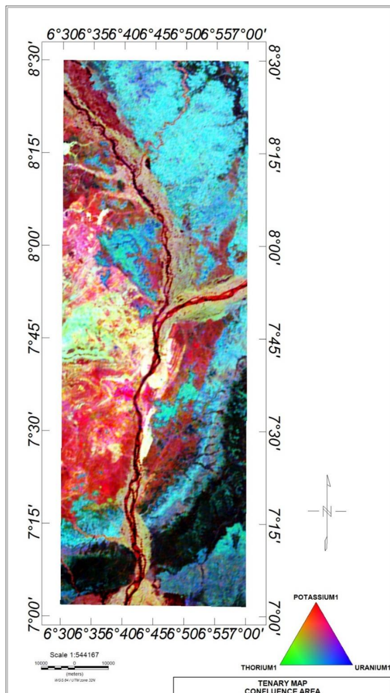
Figure 8: Ternary Map of study area
