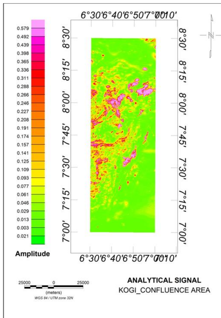
Figure 4: Analytical signal Map
